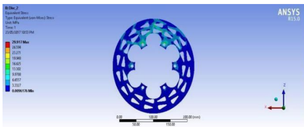
Fig 5.3 New disc 2
