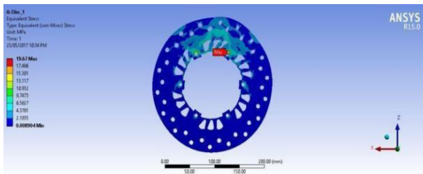
Fig 5.2 New disc 1
