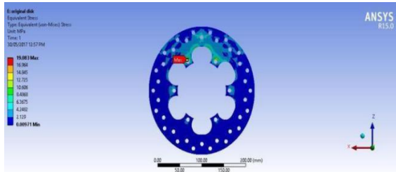
Fig 5.1 Original disc brake
