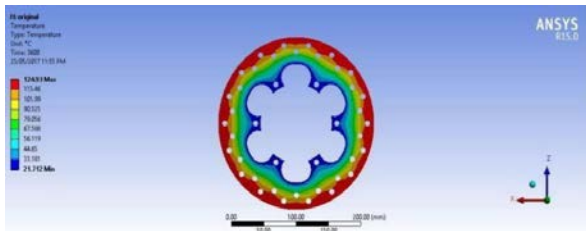
Fig 5.12 Transient thermal analysis on new disc 4
