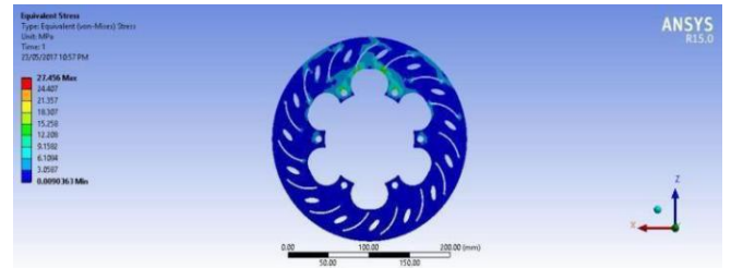
Fig 5.6 New disc 5
